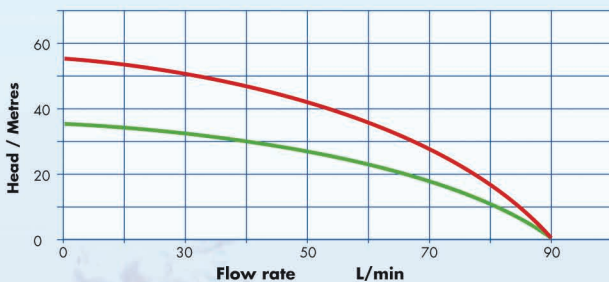
Performance Curve Multistage 900 / 1300 PC
